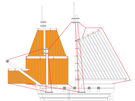
BRIGANTINE SAIL CUT-OUT
